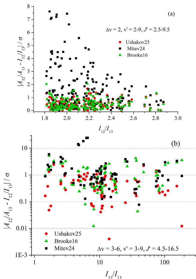
Fig. 15. Calculated-minus-observed ratios of the Einstein- A coefficients for ^{16}\text{OH} lines 1 \rightarrow 2 and 1 \rightarrow 3 emitted from a common upper level 1 divided by the experimental uncertainty, \sigma . I_{12}/I_{13} are ratios of the observed fluxes in Rayleigh emitted from the same level 1. (a), Experimental data of Brooke et al. (2016) recalculated from the laboratory spectra of Abrams et al. [312]. (b), Observational data of Noll et al. (2020). Theoretical data: circles, Ushakov et al. (2025) [310] (used for HITRAN2024); triangles, Brooke et al. [308] (used in HITRAN2016 [16] and HITRAN2020 [17]); squares, Mitev et al. (2024) [313] (used for ExoMol [218]).
