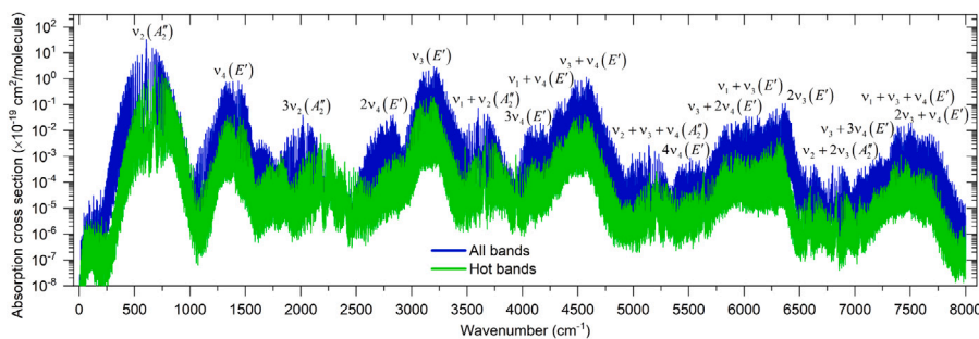
Fig. 28. Absorption cross section of ^{12}\text{CH}_3(\bar{X}^2A'') at T = 296\text{ K} simulated with the step of 0.01\text{ cm}^{-1} using a Lorentzian profile function with \text{HWHM} = 0.07\text{ cm}^{-1} . The vibrational assignment of the strongest cold bands (within a certain spectral region) is displayed.
