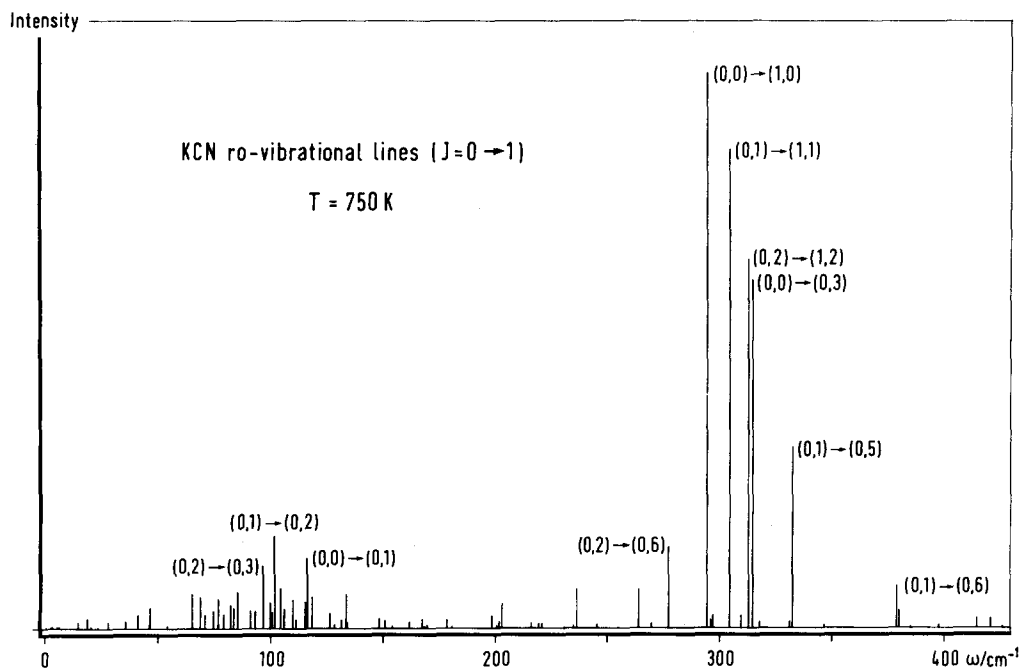
FIG. 4. Relative absorption coefficients of KCN for rovibrational J = 0 \rightarrow 1 transitions between the lowest ten vibrational ( \nu_s, \nu_b ) levels. Energy level populations are given by the Boltzmann distribution at a temperature T = 750 K.
