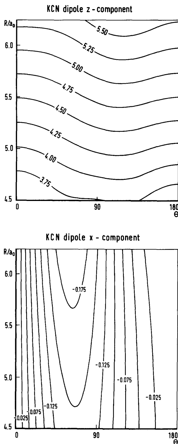
FIG. 1. Contour diagrams for the dipole components of KCN. R is the distance from the CN center of mass to K, and \theta the angle R makes with r(\text{CN}) , measured from C. Dipole values in ea_0 .
