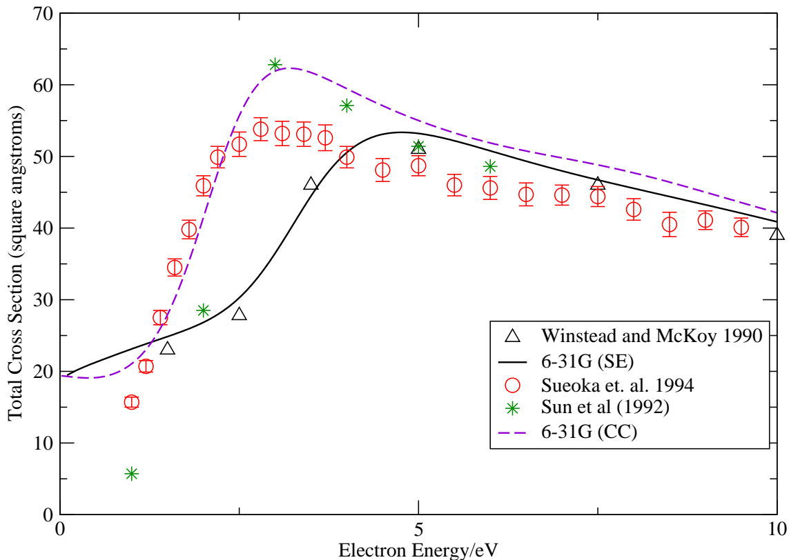
Figure 12. Total cross section for electron-silane collisions. Curves are for the SE and CC models of this work, see text for details. Points are the measurements of Sueoka et al [47], the SE calculations of Winstead and McKoy [51] and the polarised target calculation of Sun et al [53].
