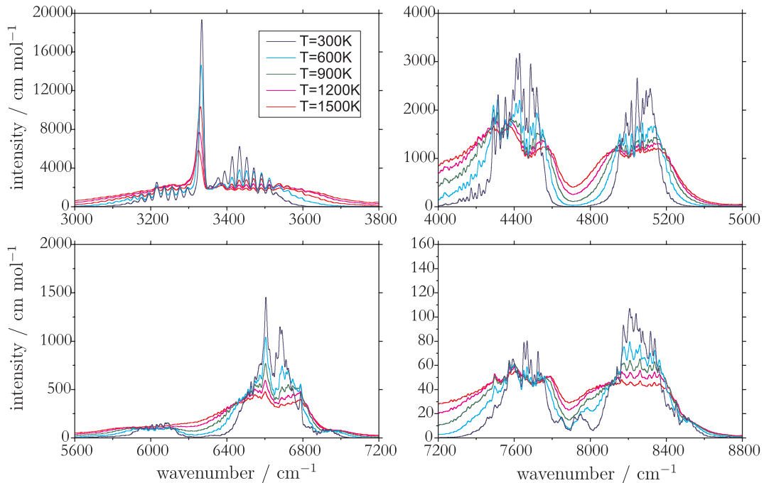
Figure 5. BYTe absorption spectra of \text{NH}_3 for T = 300, 600, 900, 1200 and 1500 K, convoluted with a Gaussian profile, \text{HWHM} = 5 \text{cm}^{-1} : the 3-, 2-, 1.5- and 1.25- \mu\text{m} regions.
