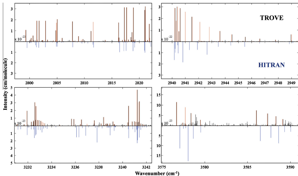
Fig. 6. HITRAN (lower) versus TROVE (upper), with matched transitions highlighted in red, for the region P = 3 . (For interpretation of the references to color in this figure legend, the reader is referred to the web version of this article.)
