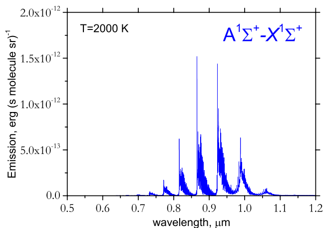
Figure 13. Emission spectrum of CaO at T = 2000 K, A^1\Sigma^+ - X^1\Sigma^+ band (Gaussian profile, HWHM = 1 \text{ cm}^{-1} ).
