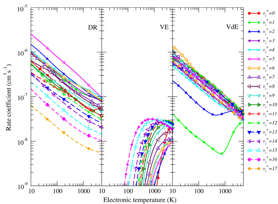
Graph 7. Global (sum over all the possible final states) Maxwell rate coefficients for dissociative recombination (DR), vibrational excitation (VE) and vibrational de-excitation (VdE).
