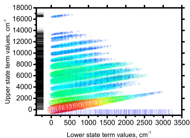
Fig. 1. The lower-state energies of the experimental ortho - \text{H}_2^{32}\text{S} transitions used in this work, against corresponding upper-state energies. The vertical bars along the horizontal-axis show the lower-state energies, while the horizontal bars along the vertical-axis give the upper-state energies. Each circle represents a particular transition, with the size proportional to the log of NumTrans, the number of transitions supporting the upper state. This value ranges from 1 (dark blue) to 404 (red). (For interpretation of the references to colour in this figure legend, the reader is referred to the web version of this article.)
