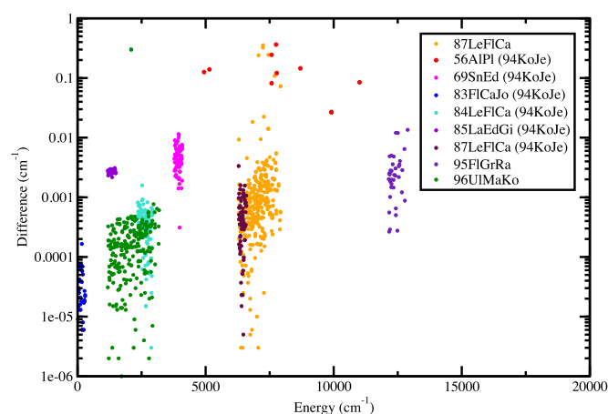
Fig. 2. Deviations in \text{cm}^{-1} between energy levels from this work and: 94KoJe [78] (see Table 7), 95FIGrRaSt [79], 87LeFIcAr [76], 96UIMaKoAl [47]. Note the logarithmic vertical-axis.
