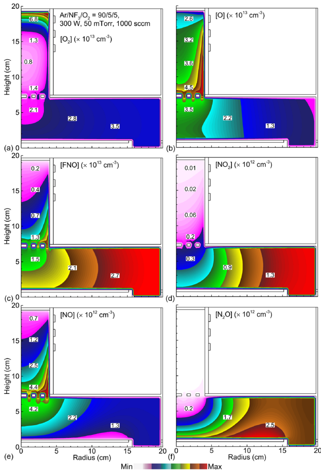
Fig. 5. (Color online) Time averaged densities of (a) \text{O}_2 , (b) \text{O} , (c) \text{FNO} , (d) \text{NO}_2 , (e) \text{NO} , and (f) \text{N}_2\text{O} in a downstream etch system with a RPS driven by inductively coupled power. Operating conditions: \text{Ar}/\text{NF}_3/\text{O}_2 = 90/5/5 , 50 mTorr, 1000 sccm, 300 W, and 10 MHz.
