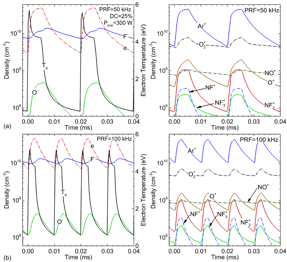
FIG. 15. (Color Online) Time variations for the volume averaged electron density, electron temperature, and ion densities in a downstream etch system with a RPS driven by pulsed inductively coupled power with PRF of (a) 50 kHz and (b) 100 kHz. Operating conditions: Ar/NF 3 /O 2 = 90/5/5, 50 mTorr, 1000 sccm, PPA power: 300 W, PRF = 50, 100 kHz, and DC = 25%.
