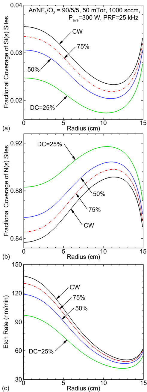
Fig. 17. (Color Online) Pulse averaged fractional coverage of (a) Si and (b) N subsites at the wafer surface and (c) etch rates of silicon nitride in a downstream etch system with a RPS driven by pulsed inductively coupled power. Operating conditions: Ar/NF 3 /O 2 = 90/5/5, 50 mTorr, 1000 sccm, PPA power: 300 W, PRF = 25 kHz, and DC = 25%–100%.
