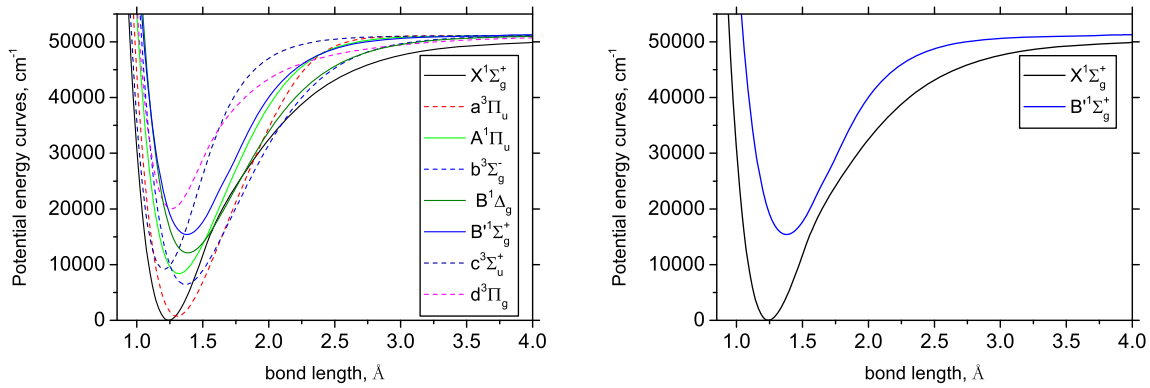
Figure 2. The eight refined potential energy curves of C_2 (left) and the avoided crossing between the X^1\Sigma_g^+ and B'^1\Sigma_g^+ states in the adiabatic representation (right).
