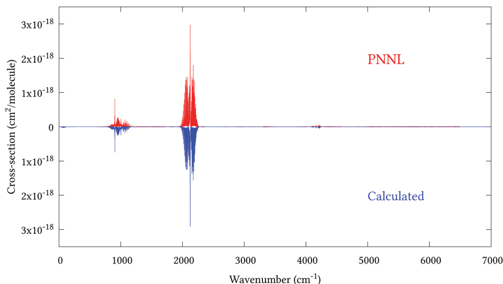
Fig. 5 Overview of synthetic J = 0\text{--}30 spectrum recorded at 298.15 K compared to PNNL. 0–7000 \text{cm}^{-1} region.
