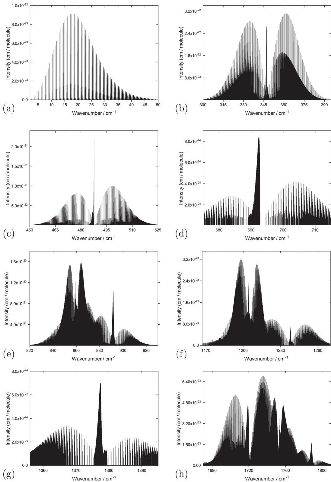
Figure 4. Stick spectra for the main \text{PF}_3 absorption bands at 296 K. (a) is pure rotational band, (b),(c) and (e) are fundamental bands and (d),(f),(g) and (h) are overtone and combination bands. Details of each band are given in main text.
