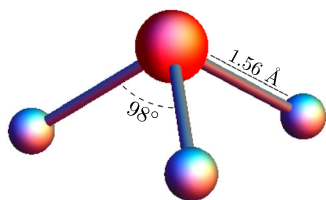
Figure 1. Equilibrium configuration of PF 3 .
