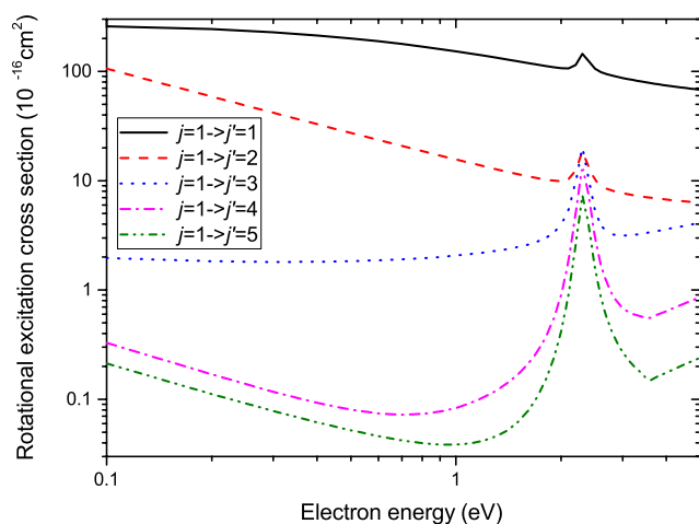
FIG. 37. Rotational excitation cross sections of the NO 2 molecule computed in this study.
