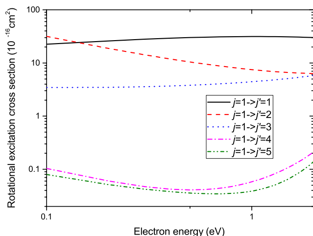
FIG. 23. Rotational excitation cross sections of the N_2O molecule computed using the UK R-matrix 88,89 and the POLYDCS 90 codes.
