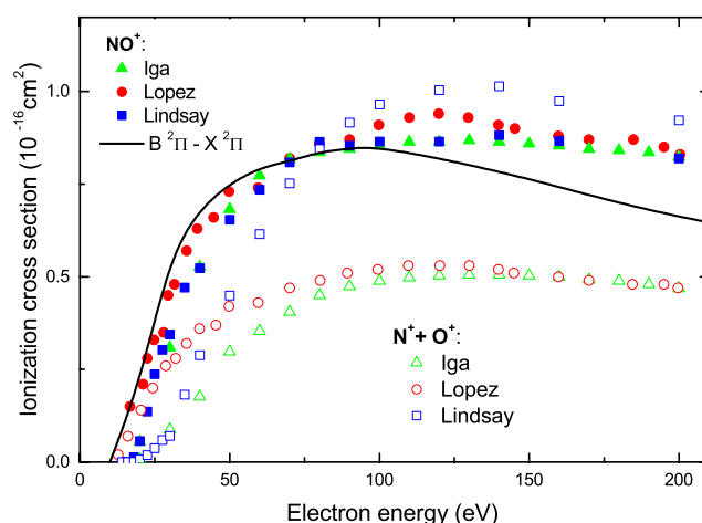
FIG. 31. Partial ionization of \text{N}_2\text{O} into \text{NO}^+ and (\text{N}^+ + \text{O}^+) . Experimental data from Refs. 27, 30, and 31. The optical emission from \text{NO}^+ for the \text{B}^2\Pi \rightarrow \text{X}^2\Pi transition 111 (normalized by a factor of 40 to Lindsay et al. 's 27 \text{NO}^+ signal at 70 eV) is also shown.
