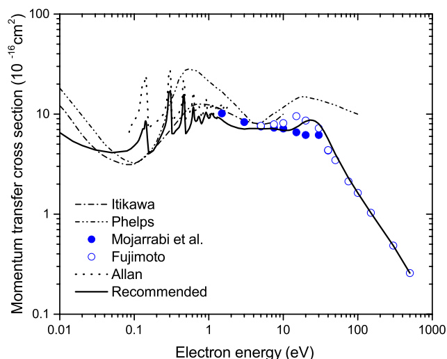
FIG. 6. Momentum transfer cross section of NO. Dashed and single dotted line, Itikawa; 41 dashed and double dotted line, Phelps; 42 solid circle, Mojarrabi et al. ; 37 open circle, Fujimoto and Lee; 40 dotted line, Allan's 24 DCS times 4\pi ; and solid line, recommended.
