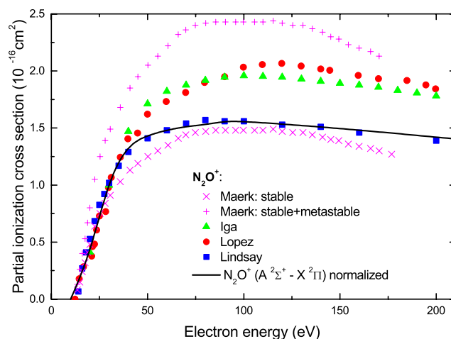
FIG. 30. Experimental 27,30,31,65 partial ionization for the parent ion \text{N}_2\text{O}^+ . The optical emission for the \text{A}^2\Sigma^+ \rightarrow \text{X}^2\Pi transition 111 (normalized by a factor of 4 to Lindsay et al. 's 27 \text{N}_2\text{O}^+ signal at 100 eV) is also shown.
