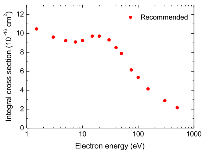
FIG. 5. Recommended elastic ICS for NO.
