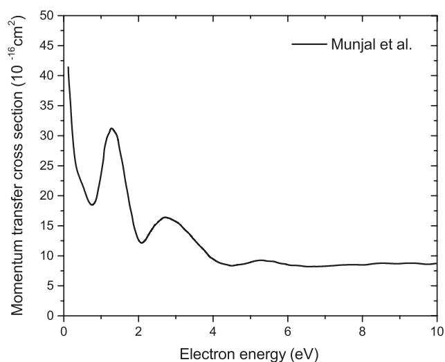
FIG. 36. Momentum transfer cross section of the NO 2 molecule computed using the R-matrix method by Munjal et al. 123
