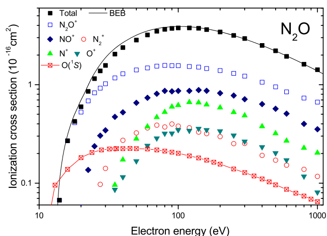
FIG. 32. Recommended cross sections for ionization of N_2O are based on Lindsay et al. 27 measurements and are the same as given by Lindsay and Mangan in their review. 27 The cross section for the formation of a neutral oxygen atom O in the ^1S_0 electronic state measured by LeClair et al. 60 is also given: this comparison makes clear that the formation of the O atom is not a “coproduct” of ionization. BEB model by Kim et al. 67 The uncertainties are \pm 5\% on total ionization and N_2O^+ , \pm 10\% on NO^+ and N^+ , and \pm 15\% on N_2^+ and O^+ partial ionization cross sections. 27
