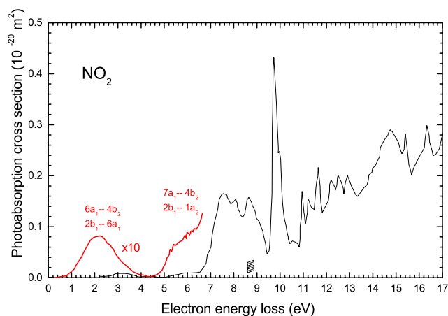
FIG. 38. Zero-angle electron-scattering energy loss spectra in NO 2 from experiments by Au et al. 127 The ionization threshold is 9.586 \pm 0.002 \text{ eV} for NO 2 .
