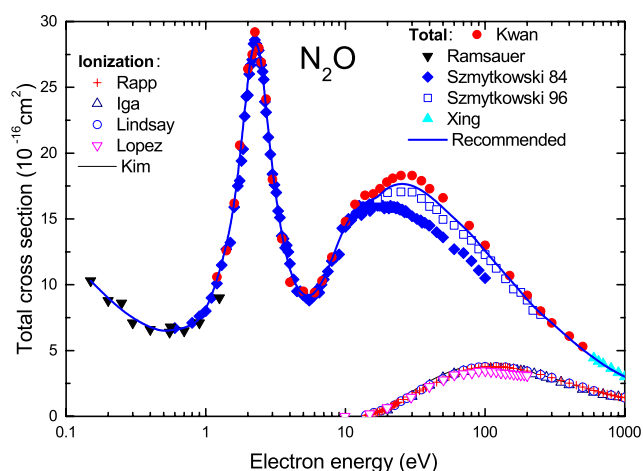
FIG. 19. TCS's for electron scattering on nitrous oxide, N_2O . Experimental absolute TCS's are from Ref. 33—full circles (digitalized from their figure), from Ref. 71—inverted triangles, Refs. 72 and 74—full diamonds, Ref. 21—open squares, and Ref. 35—full triangles. The thick line represents our recommended TCS. Ionization ICS—experiments: Rapp and Englander-Golden, 28 Iga et al. , 30 Lindsay et al. , 27 and Lopez et al. , 31 BEB model by Kim et al. 67
