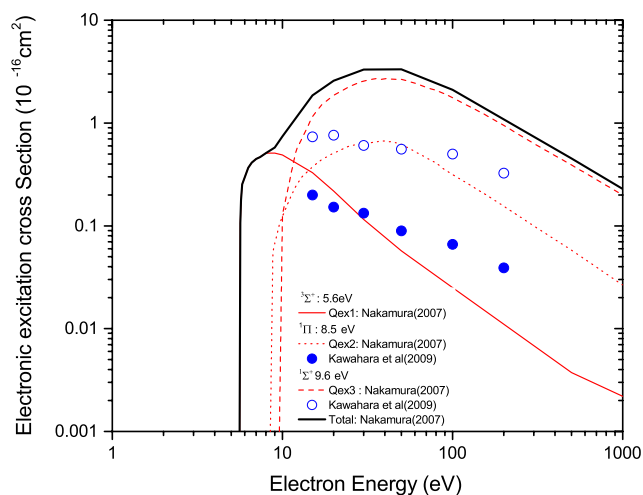
FIG. 28. Electronic excitation cross sections of \text{N}_2\text{O} . Closed and open circles, ICS 101 for excitations of \text{C}^1\Pi and \text{D}^1\Sigma^+ states, respectively; three thin curves, swarm-derived excitation cross sections whose excitation threshold are assumed to be 5.6 eV (the value assigned to ^3\Sigma^+ ), 8.5 eV ( \text{C}^1\Pi ), and 9.6 eV ( \text{D}^1\Sigma^+ ), respectively; thick solid curve, sum of the swarm-derived cross sections.
