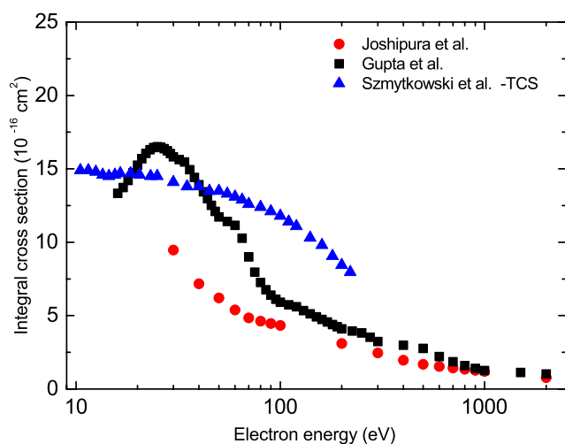
FIG. 35. Recommended elastic ICS of Joshipura et al. , 122 compared with the values computed by Gupta et al. , 120 and TCS measured by Szymtkowski et al. , 119
