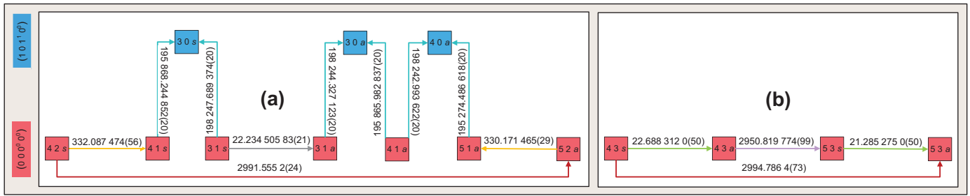
Fig. 5. Highly accurate frequency determinations for lines at 2991.555 [panel (a)] and 2994.786 GHz [panel (b)] NASEM frequencies (see also Table 4). The J K inv rotational labels within the squares represent rovibrational states, whose (v_1 v_2 v_3 v_4) vibrational labels are indicated in the left-hand-side legend with different colors. Transitions designated with orange, cyan, gray, brown, green, and purple arrows are results from 88TaEnHi [111], 16TwHaSe [30], 70KuWo [44], 83PoMa [54], 75PoKa [110], and 10YuPeDrSu [81], respectively. Lines are augmented with their experimental frequencies (in GHz) and the uncertainties of the last few frequency digits given in parentheses. In both cases (a) and (b), the brown connectors of 83PoMa denote the best available observations for the corresponding transitions. Employing the Ritz principle successively, the following empirical predictions are derived from the two underlying network paths: 332.087\,474 + 195\,868.244\,852 - 198\,247.689\,374 + 22.234\,505\,83(21) + 198\,244.327\,123 - 195\,865.982\,837 + 198\,242.993\,622 - 195\,274.486\,618 - 330.171\,465 \approx 2991.557\,284 and 22.688\,312\,0 + 2950.819\,774 + 21.285\,275\,0 \approx 2994.793\,361 GHz. These two estimates can be associated with the uncertainties of \sqrt{56^2 + 20^2 + 20^2 + 0.21^2 + 20^2 + 20^2 + 20^2 + 20^2 + 29^2} \approx 80 and \sqrt{5^2 + 99^2 + 5^2} \approx 99 kHz, respectively. These path-based frequencies, together with the MARVEL-predicted values utilizing the full network information [2991.557 31(11) and 2994.793 39(13) GHz, see Table 4], are at least 10 times more accurate than the direct brown links of 83PoMa [54]. (For interpretation of the references to color in this figure legend, the reader is referred to the web version of this article.)
