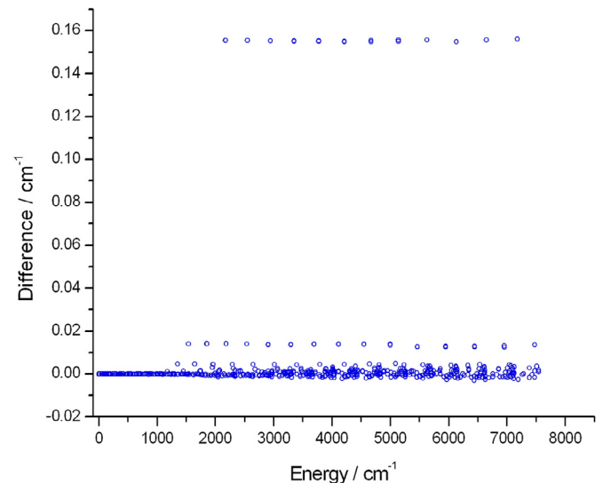
Fig. 2. Comparison of the empirical ground-vibrational-state energies of ^{14}\text{NH}_3 of this study with their 18PeYuPeSu [82] counterparts.
