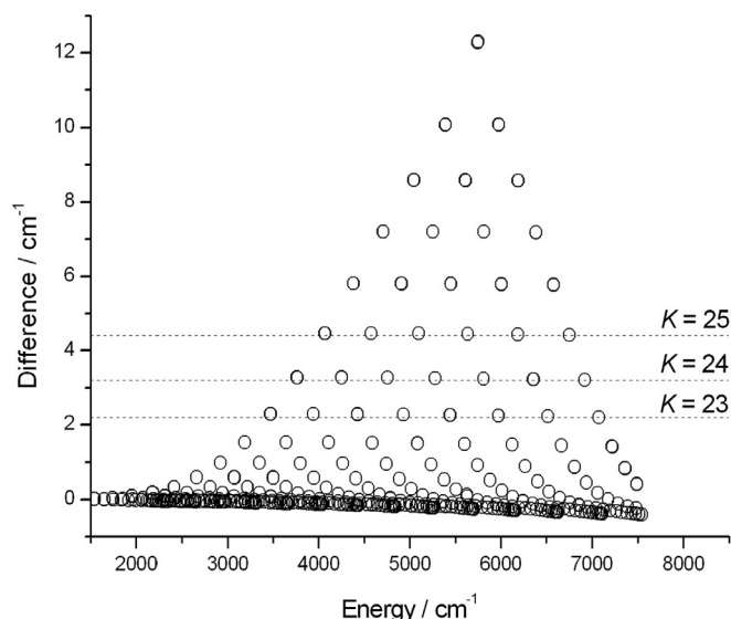
Fig. 3. Effective Hamiltonian model energies of 18PeYuPeSu [82] compared to their CoYuTe [71] first-principles counterparts above J = 15 on the ground vibrational state of ^{14}\text{NH}_3 .
