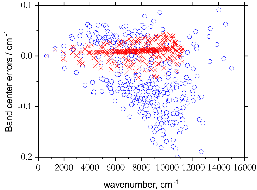
Figure 1. Blue circles: Average ro-vibrational errors for 337 vibrational ( J = 0 ) states \tilde{E}_\lambda^{\text{H}} - \tilde{E}_\lambda^{\text{T}} (HITRAN–TROVE) term values for J \leq 40 , which were used as band centre corrections (see the text). Red crosses: Average residuals for the ro-vibrational CO 2 term values (for J \leq 40 ) between TROVE (before the band centre correction) and calculations from Zak et al. (2016) using DVR3D and the same PES Ames-2016 for 294 vibrational states.
