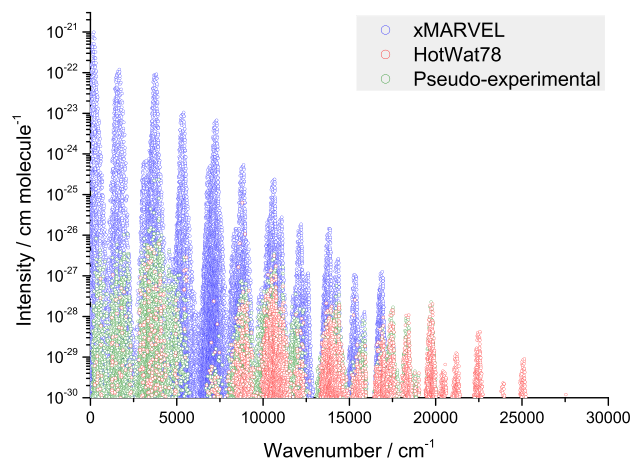
FIG. 13. Room-temperature one-photon, dipole-allowed \text{H}_2^{17}\text{O} linelist up to 30 000 \text{cm}^{-1} , with an intensity cutoff of 10^{-30} \text{cm molecule}^{-1} , based on xMARVEL, HotWat78, 128 and PE line positions. In the cases where a wavenumber is provided by more than one dataset, only the most accurate value is retained in the figure, following the xMARVEL > HotWat78 > PE accuracy relations. The intensities are taken from Ref. 128.
