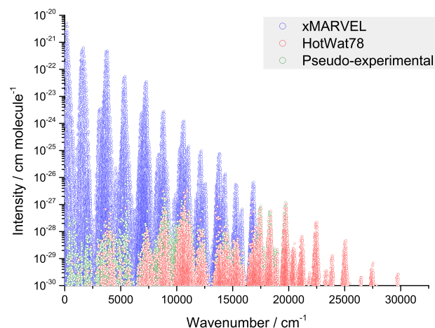
FIG. 15. Room-temperature one-photon, dipole-allowed \text{H}_2^{18}\text{O} linelist up to 30 000 \text{cm}^{-1} , with an intensity cutoff of 10^{-30} \text{cm molecule}^{-1} , based on xMARVEL, HotWat78, 128 and PE line positions. In the cases where a wavenumber is provided by more than one dataset, only the most accurate value is retained in the figure, following the xMARVEL > HotWat78 > PE accuracy relations. The intensities are taken from Ref. 128.
