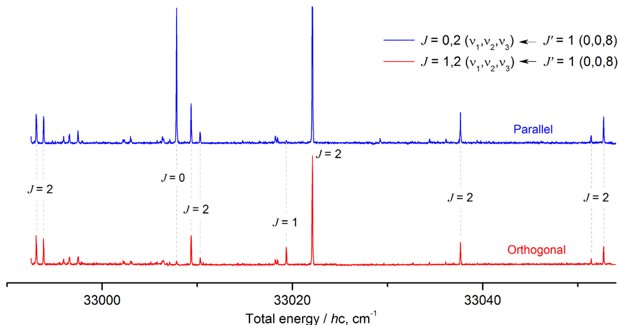
Fig. 2. Photofragment spectra of HD 16 O from the gateway state (in normal mode vibrational notation) [25347.43 cm -1 , 1 0,1 (0,0,8)] to the terminal vibrational state ( \nu_1, \nu_2, \nu_3 ) with either J=0,2 (blue) or J=1,2 (red) for parallel and orthogonal polarization of the P_3 laser respectively (see text for details). Corresponding J -notations of the observed transitions are provided on the plot.
