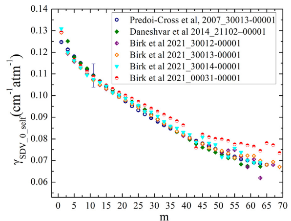
Fig. 6. The self-broadening parameters for \text{CO}_2 transitions at 296 K using the SDV profile. The values by Predoi-Cross et al. [176] are compared with the measurement of Ref. [177]. The Birk et al. [153] values are also presented for different bands.
