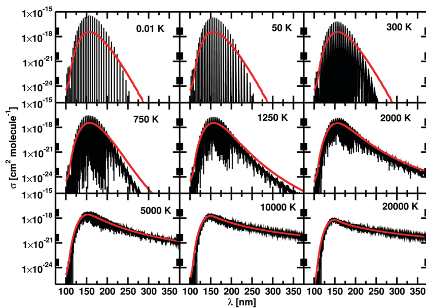
Fig. 5 Unsmoothed (black) and smoothed (red) cross sections of HCl at different temperatures. With the increase of temperature from 0.01 K to 20 000 K, the filling between lines becomes smaller up to the point that a continuous spectrum is recovered. The unsmoothed and smoothed spectra coincide from 2000 K. The number of accessible rovibrational states increase with the temperature, reducing the difference between the unsmoothed and smoothed data. This effect is evident at long wavelengths, above 225 nm.
