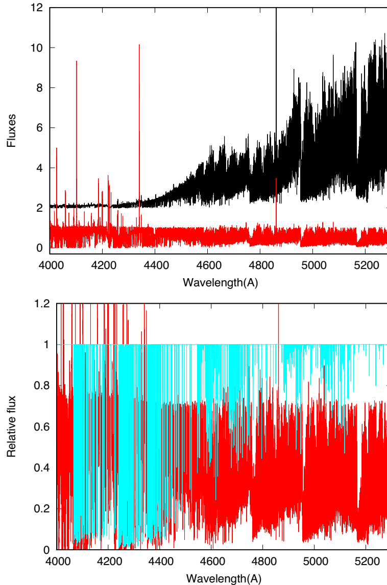
Figure 1. Top panel: Observed HARPS s1d spectrum of Proxima Cen (black line) and the same spectrum reduced to continuum/pseudo-continuum (red line). Bottom panel: A comparison of the theoretical R_f (cyan line) and reduced to pseudo-continuum observed spectrum (red line).
