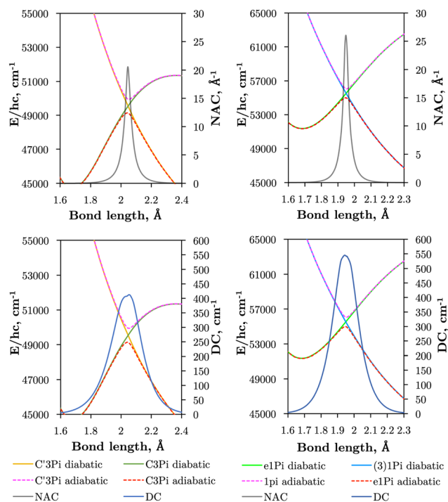
Fig. 8 Illustration of the avoided crossings between e^1\Pi – (3)^1\Pi and (right panels) and C^3\Pi – C^3\Pi states of SO (left panels) where adiabatic PECs are presented as dashed lines and diabatic ones in solid lines. Superimposed are the DCs ( V_{12}^a , bottom panels), and NACs ( \phi_{ij}^a , top panels).
