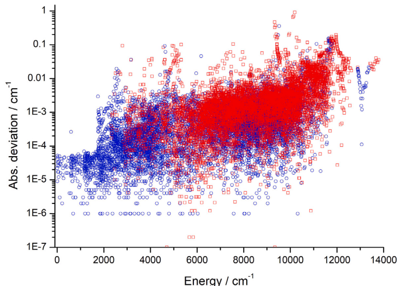
Fig. 4. Absolute deviations between the empirical (MARVEL) energy levels of this study and those of the NOSL-296 line list [179]; see text for the subset of NOSL-296 levels which could be utilized for this comparison. Blue circles indicate states with MARVEL energies determined by at least three measured lines, while the red squares correspond to the states with MARVEL energies determined by one or two measured lines.
