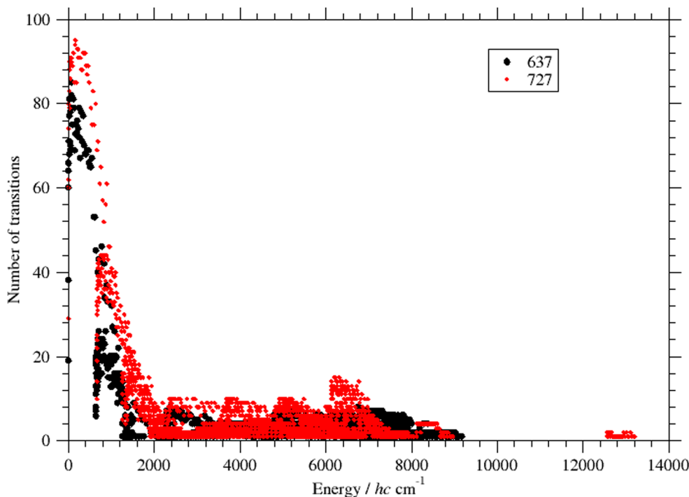
Figure 2. The number of transitions incident to each energy level versus the empirical rovibrational energy level values determined in this study for ^{16}\text{O}^{13}\text{C}^{17}\text{O} (637, black dots) and ^{17}\text{O}^{12}\text{C}^{17}\text{O} (727, red dots).
