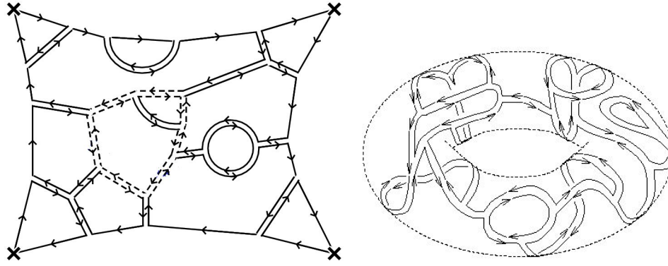
FIGURE 11.1: (a) ribbon graphs on a planar topological space (or sphere), (b) ribbon graphs on a toroidal topological space [230]
