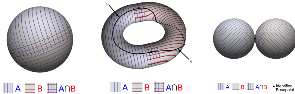
FIGURE 10.2: (a) Normal vacuum, topologically represented as a sphere, with direct vacuum entanglement on the intersection region (b) E.R. bridge with the topology of a torus. Entanglement associated to the intersection (c)homology, isomorphic to two separated circles. The one-chains u and v with boundaries in the intersection can be glued to form a 1-cycle u + v . (c) Wedge sum of two spheres tangent at one point with entanglement associated to space homological to a single point. The associated 0-degree homology is the coefficient group of the theory according to the Eilenberg-Steenrod axioms
