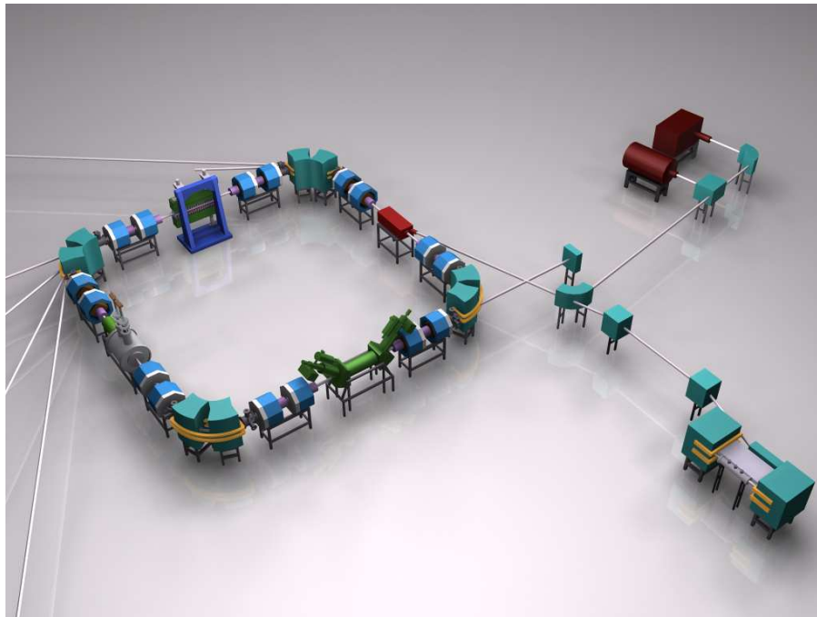
Figure 1.3: ASTRID (Aarhus STorage RIng in Denmark): a dual-mode ring which can store electrons or ions of either polarity ( http://www.isa.au.dk/animations/pictures/pic-index.html ).
