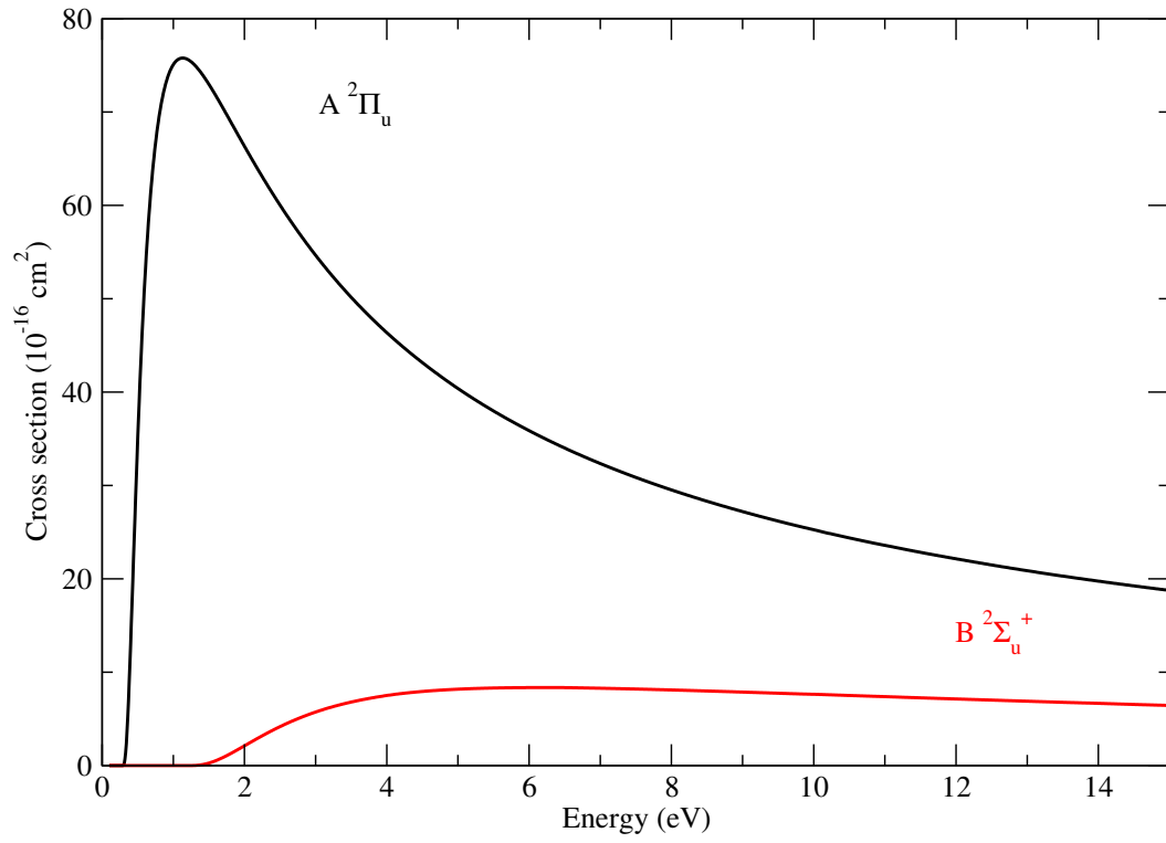
Figure 6.11: Electronic excitation cross sections to the A \ ^2\Pi_u and B \ ^2\Sigma_u^+ states with Born correction for model 4 with \alpha_0=0.17 and \beta=1.3 .
