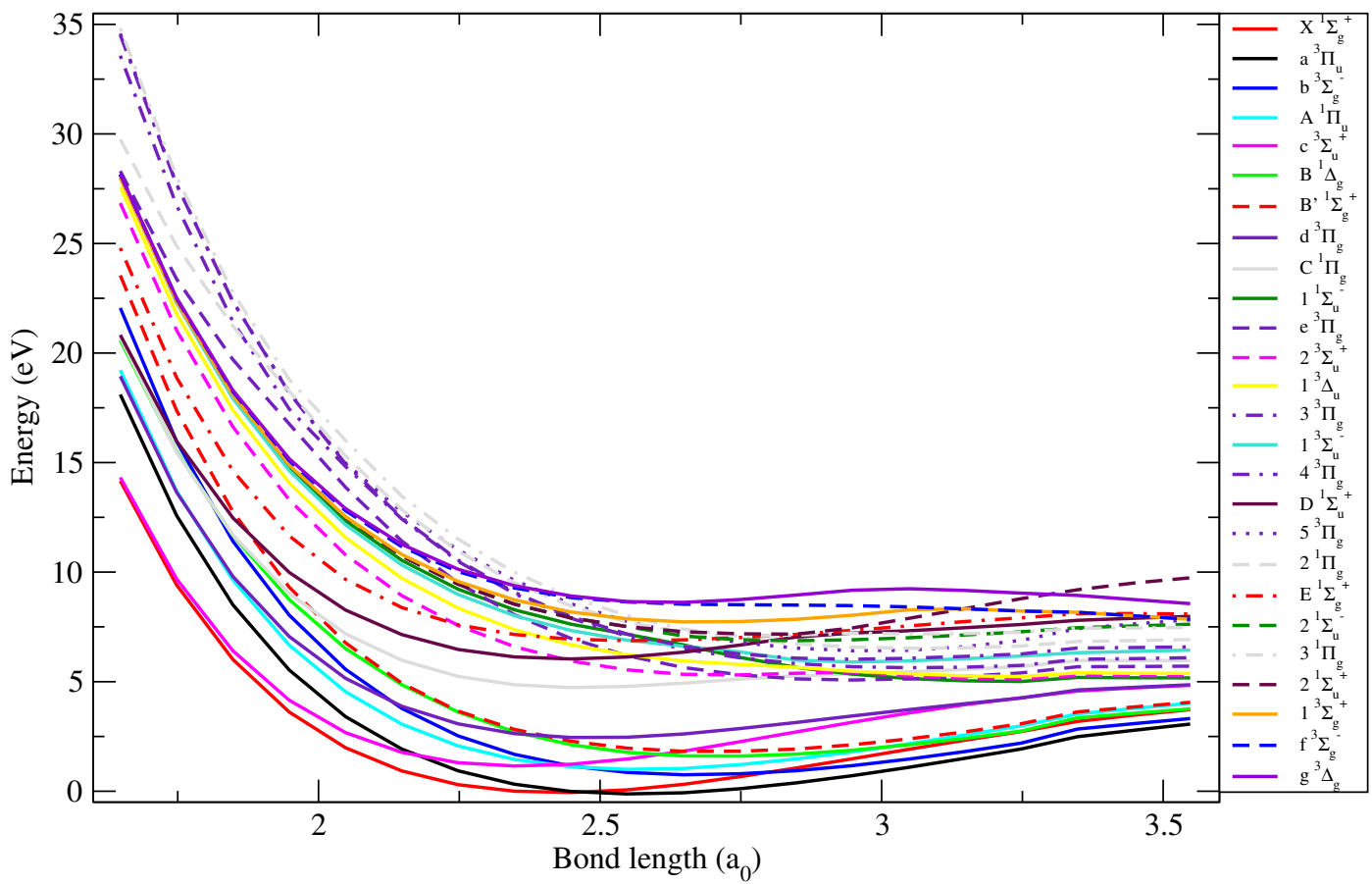
Figure 4.1: Potential energy curves for the 26 states of C_2 used in the calculations.
