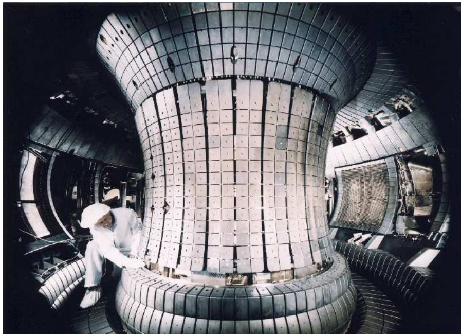
Figure 1.1: The ASDEX Upgrade divertor tokamak: inside view of the vacuum vessel with divertor II.
