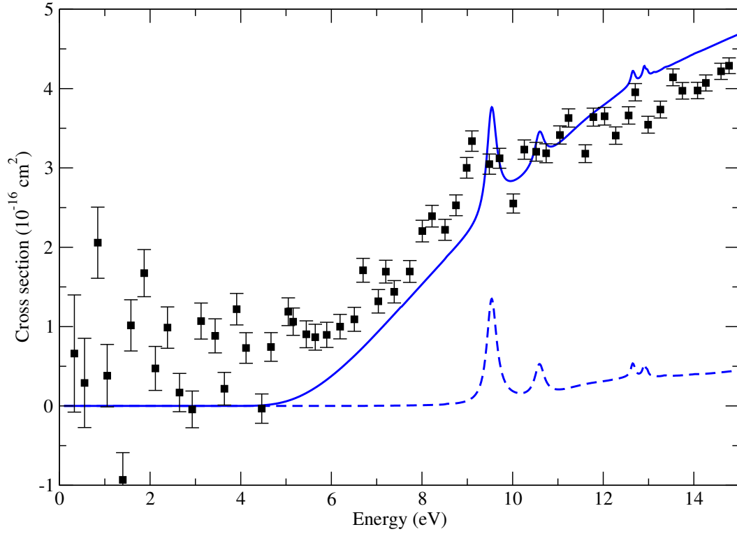
Figure 6.13: Ionisation cross sections of C_2^- for model 5 with \alpha_0=0.17 and \beta=1.4 . The experimental data (Pedersen et al., 1999) is indicated with full black squares (with dissociative channels); the dashed line represents cross section without Born correction and the solid line represents cross section with Born correction.
