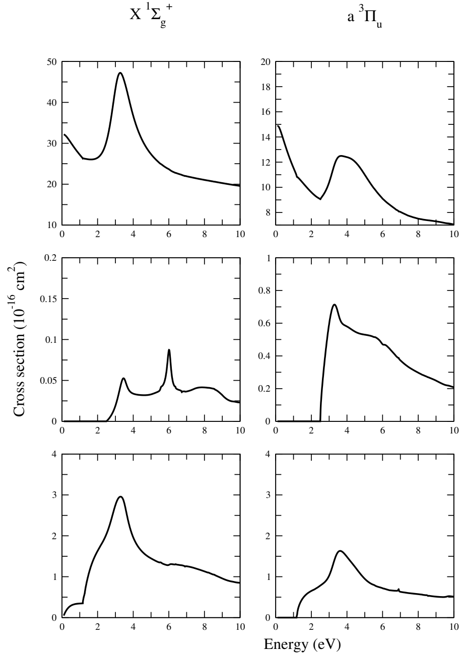
Figure 4.9: Electronic excitation cross sections from ground state ( X^1\Sigma_g^+ ) and first excited state ( a^3\Pi_u ) of C_2 at its equilibrium geometry. The first row represents the fixed-nuclei total cross sections. The second row represents cross sections for the excitation to d^3\Pi_g state. The third row represents the cross sections for the electron impact excitation to the four electronic states of C_2 lying between the two initial states and d^3\Pi_g state.
