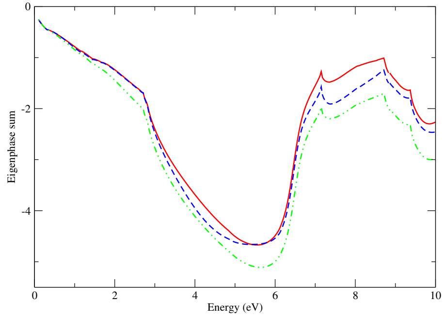
Figure 4.2: The eigenphase sums (in radians) for {}^2A_g ( {}^2\Sigma_g^+ + {}^2\Delta_g ) symmetry of the low-energy electron collisions with C_2 . The solid red line represents the eigenphase sum calculated for R -matrix radius of a=10 a_0 and continuum basis of Faure et al. (2002); the dashed blue line represents the eigenphase sum calculated for R -matrix radius of a=13 a_0 and continuum basis of Faure et al. (2002) and the dot-dashed green line represents the eigenphase sum calculated for R -matrix radius of a=10 a_0 and continuum basis of Sarpal et al. (1996).
