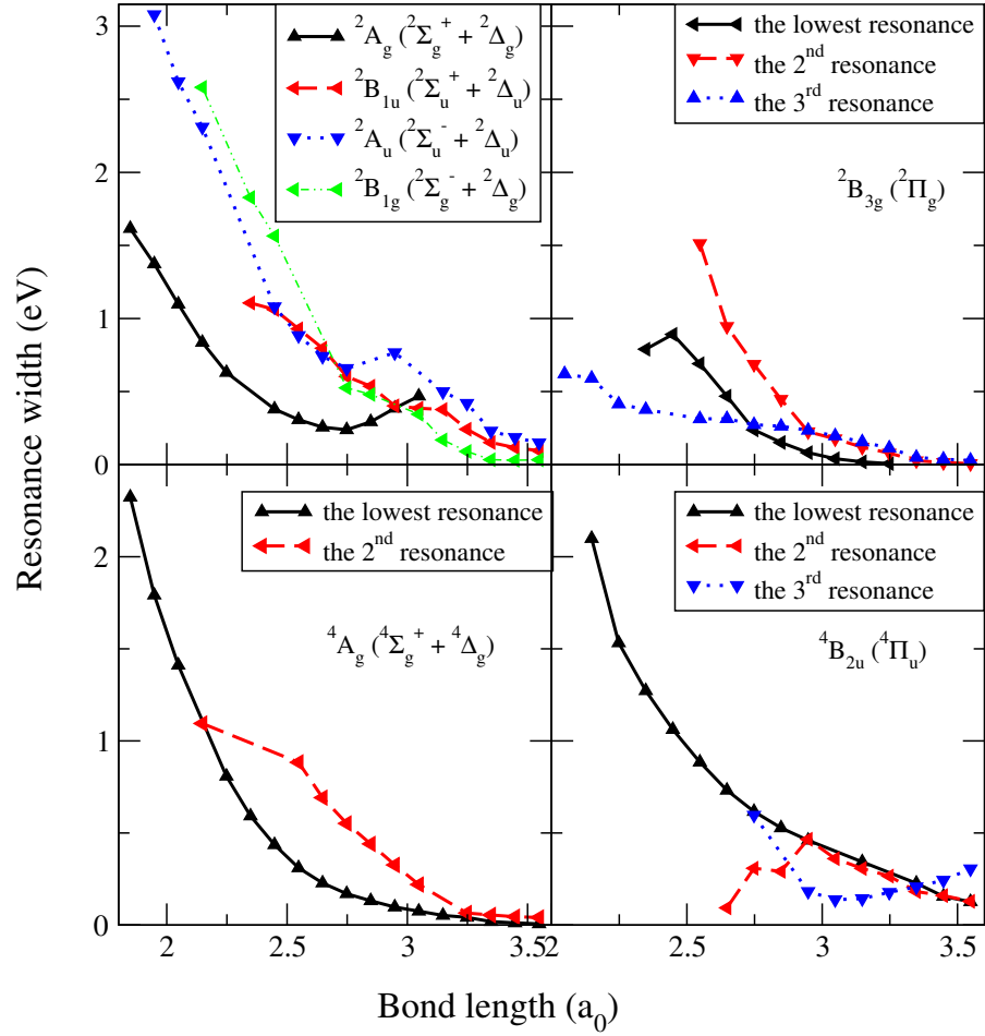
Figure 4.7: C_2^- resonance widths for ^2A_g ( ^2\Sigma_g^+ + ^2\Delta_g ), ^2B_{1u} ( ^2\Sigma_u^+ + ^2\Delta_u ), ^2B_{3g} ( ^2\Pi_g ), ^4A_g ( ^4\Sigma_g^+ + ^4\Delta_g ) and ^4B_{2u} ( ^4\Pi_u ) symmetries as a function of the bond length.
