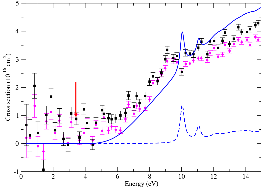
Figure 6.12: Ionisation cross sections of C_2^- for model 4 with \alpha_0=0.17 and \beta=1.4 . The experimental data (Pedersen et al., 1999) is indicated with full magenta circles (without dissociative channels) and black squares (with dissociative channels); the dashed line represents cross section without Born correction; the solid line represents cross section with Born correction and the red arrow indicate the location of the ionisation threshold.
