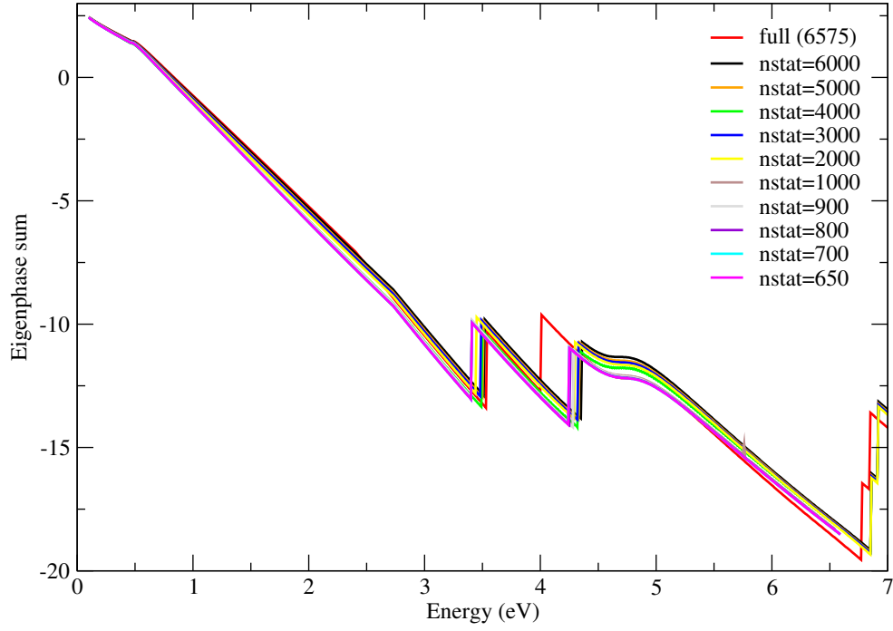
Figure 6.6: The eigenphase sums for ^2A_g symmetry of the (C_2^- + e^-) system at equilibrium geometry as a function of energy using the partitioned R -matrix method for model 4 . The different dimensions of Hamiltonian were tested as indicated in the legend.
