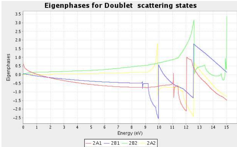
Figure 4.12: H 2 O eigenphase sums for a 10-state CC calculation
