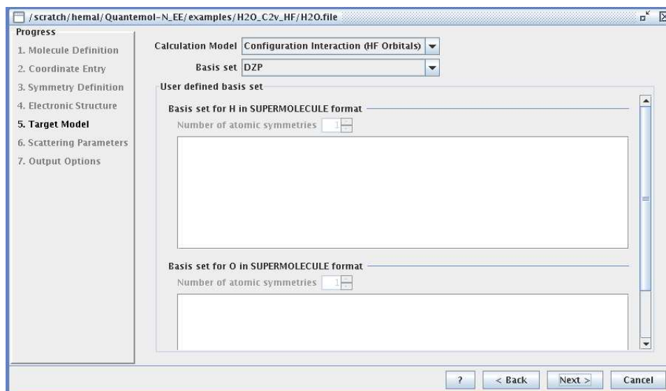
Figure 4.5: Wizard panel 5: quantum chemistry parameters
