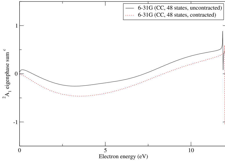
Figure 9.3: Comparison of \text{CH}_4 ^2\text{A}_1 eigenphase sum curves
