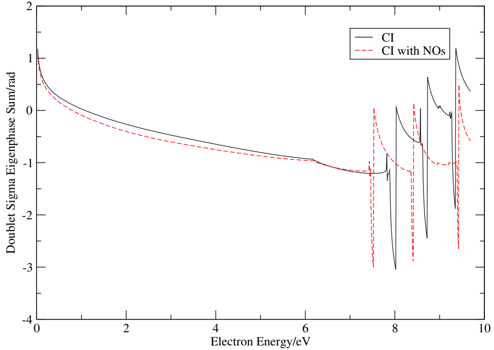
Figure 5.3: Comparison of HNC ^2\Sigma^+ eigenphase sum curve
