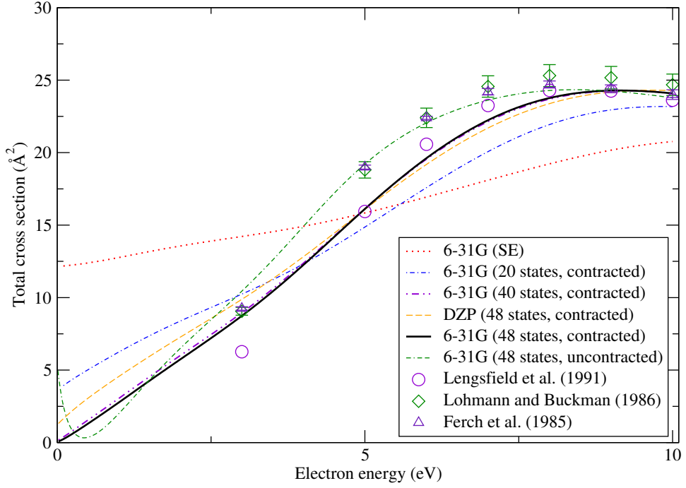
Figure 9.5: Comparison of CH 4 integral elastic cross sections
