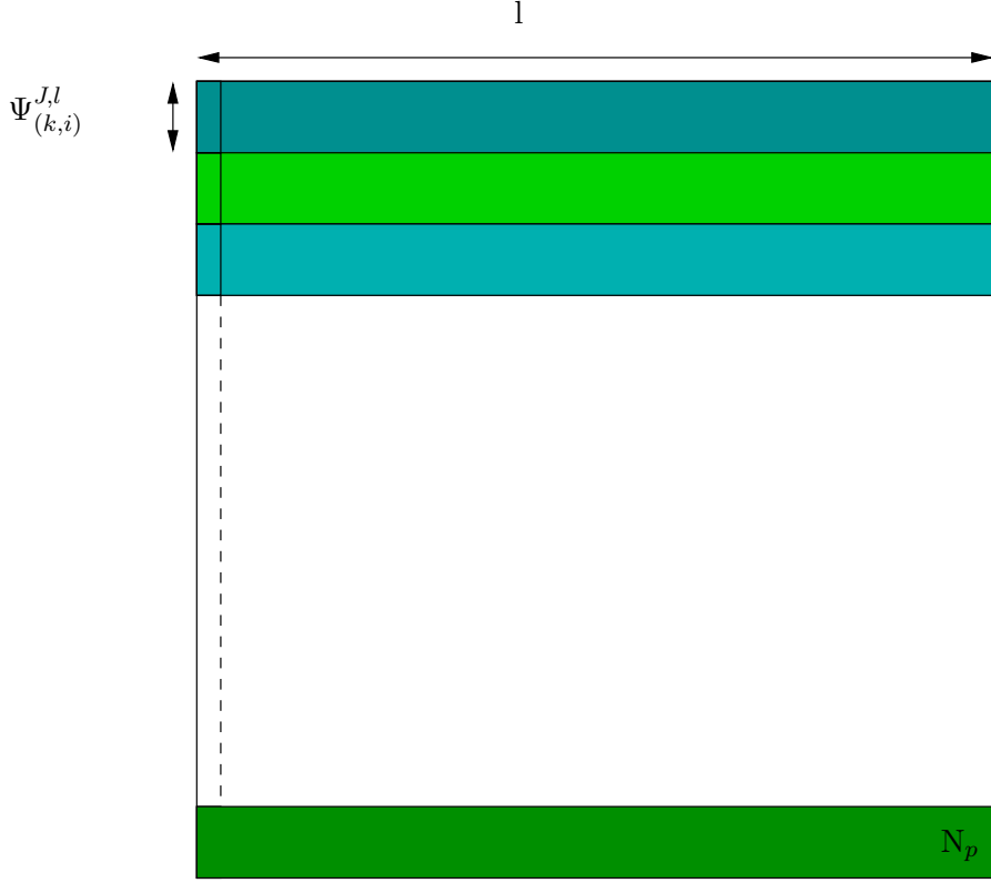
Figure 5.13: The distribution across, N_p , processors of, l , eigenvectors, \psi_{k,i}^{J,l} , produced by PARPACK [14].
