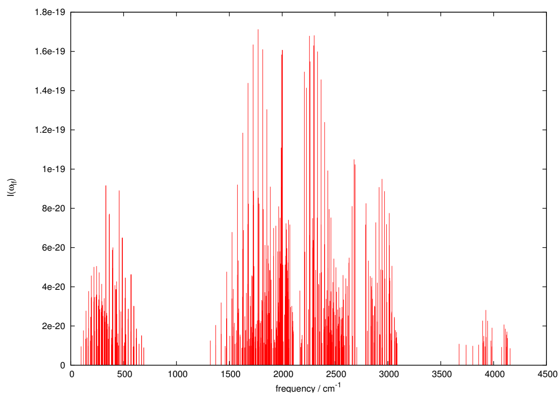
Figure 4.13: Ab initio synthetic pure rotational spectrum of \text{D}_2\text{H}^+ at 1000 K
