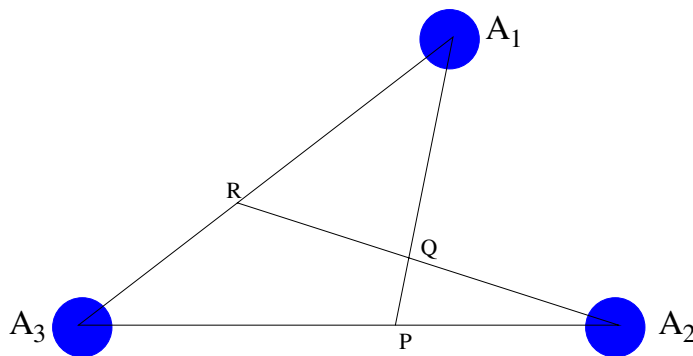
Figure 2.7: Generalised internal coordinate system for a triatomic molecule [6]: A_i represents atom i . The coordinates, r_1 , r_2 , and \theta are given by r_1 = \overline{A_2R} , r_2 = \overline{A_1P} , \theta = \angle A_1QA_2 . The positions of P and R are determined from the particular choice of coordinate system and the masses of A_i .
