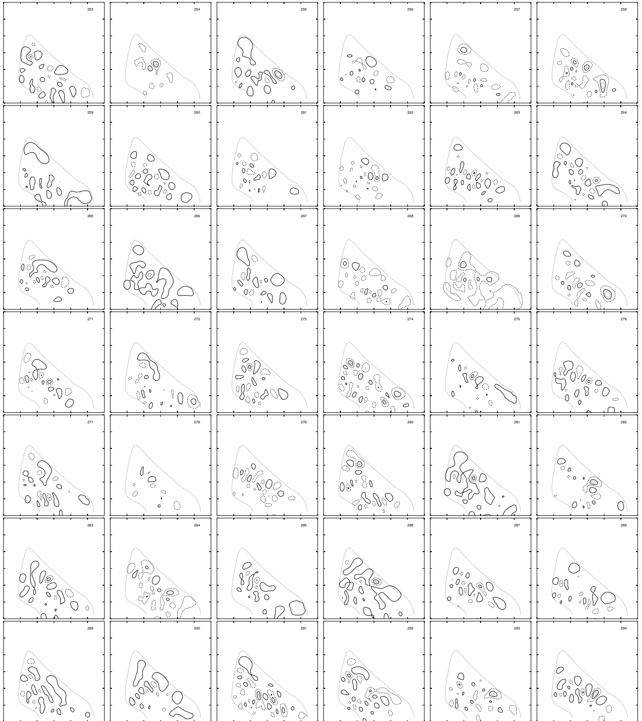
Figure 7.7: \text{H}_3^+ J = 0 even ( q = 0 ) wavefunctions in Jacobi (r_1, r_2, \theta) coordinates for states 253 to 294 with \theta taken to be 88.2^\circ . Contours are taken at 8%, 16%, 32% and 64% of the maximum amplitude. The dashed line enclosing each state indicates the classical turning point for that state. r_1 and r_2 are along the x and y axes respectively, with ranges from 0 to 6 a_0 .
