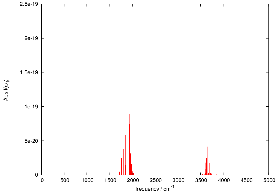
Figure 4.8: Ab initio synthetic spectrum of H_3^+ at 50 K, for J = 0 to 4 up to a frequency of 5000\text{ cm}^{-1} .
