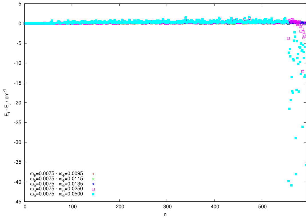
Figure 6.5: Convergence of J = 0 odd band origins with respect to the value of \omega . The points indicate the difference of the n^{th} energy level calculated using a particular value of \omega relative to that calculated with \omega = 0.0075
