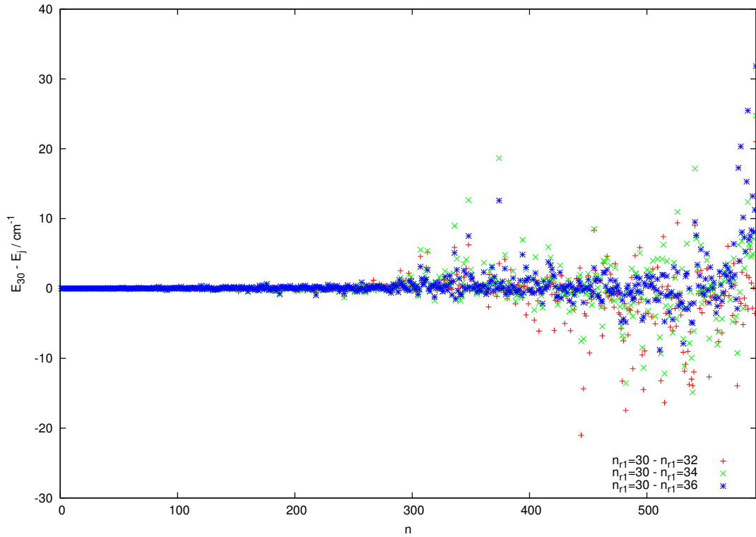
Figure 6.9: Convergence of J = 0 odd band origins with respect to the value of n_{r_1} . The points indicate the difference of the n^{th} energy level calculated using a particular value of n_{r_1} relative to that calculated with n_{r_1}
