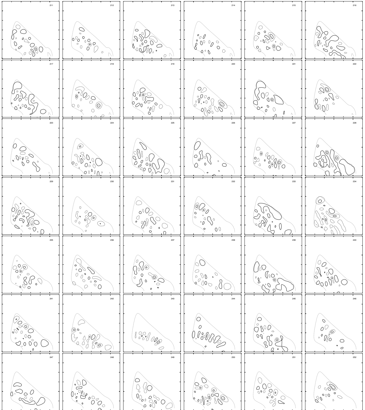
Figure 7.6: \text{H}_3^+ J=0 even ( q=0 ) wavefunctions in Jacobi (r_1, r_2, \theta) coordinates for states 211 to 252 with \theta taken to be 88.2^\circ . Contours are taken at 8%, 16%, 32% and 64% of the maximum amplitude. The dashed line enclosing each state indicates the classical turning point for that state. r_1 and r_2 are along the x and y axes respectively, with ranges from 0 to 6 a_0 .
