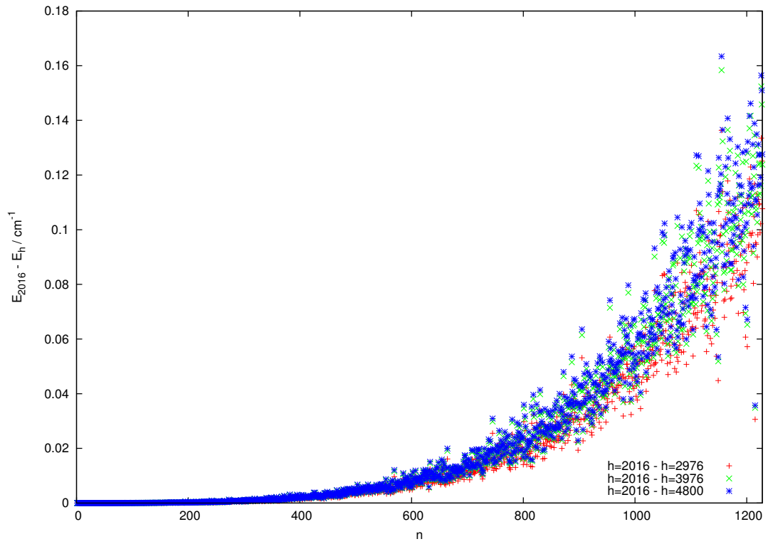
Figure 6.16: The convergence of J = 1 , odd, e states. The points indicate the difference between the n^{th} energy level calculated with h = 2016 and other values of h .
