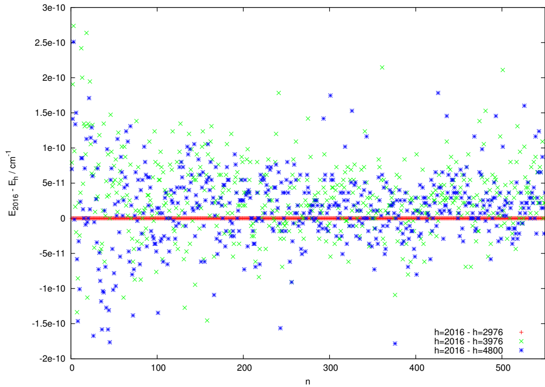
Figure 6.17: The convergence of J = 1 , odd, f states. The points indicate the difference between the n^{th} energy level calculated with h = 2016 and other values of h .
