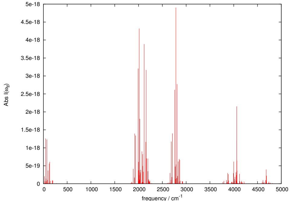
Figure 4.7: Ab initio synthetic spectrum of D_2H^+ at 50 K, for J = 0 to 4 up to a frequency of 5000\text{ cm}^{-1} . I(\omega_{if}) are explicitly calculated using the nuclear spin factors given by the symmetry assignment of energy levels.
