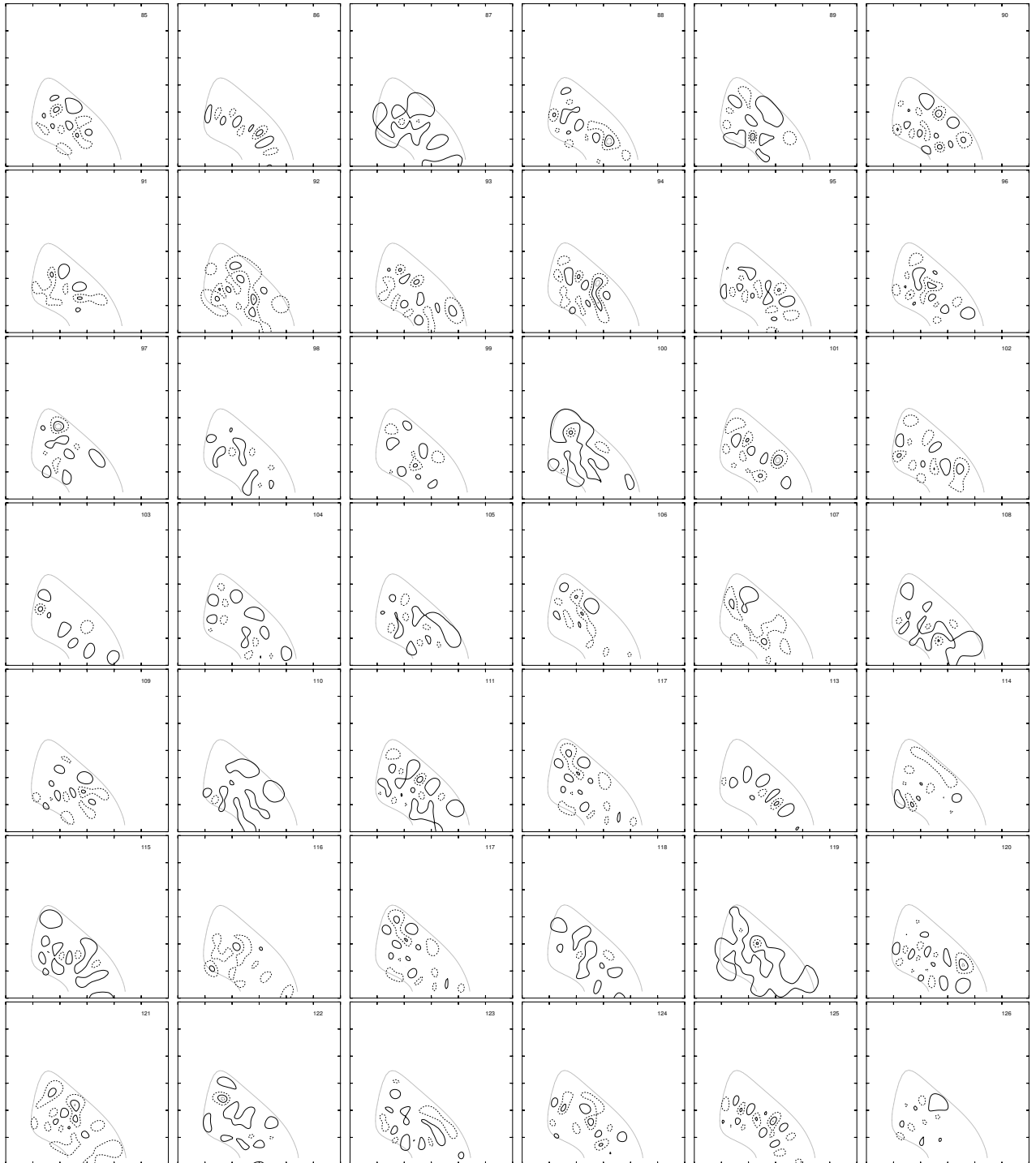
Figure 7.3: \text{H}_3^+ J = 0 even ( q = 0 ) wavefunctions in Jacobi (r_1, r_2, \theta) coordinates for states 85 to 126 with \theta taken to be 88.2^\circ . Contours are taken at 8%, 16%, 32% and 64% of the maximum amplitude. The dashed line enclosing each state indicates the classical turning point for that state. r_1 and r_2 are along the x and y axes respectively, with ranges from 0 to 6 a_0 .
