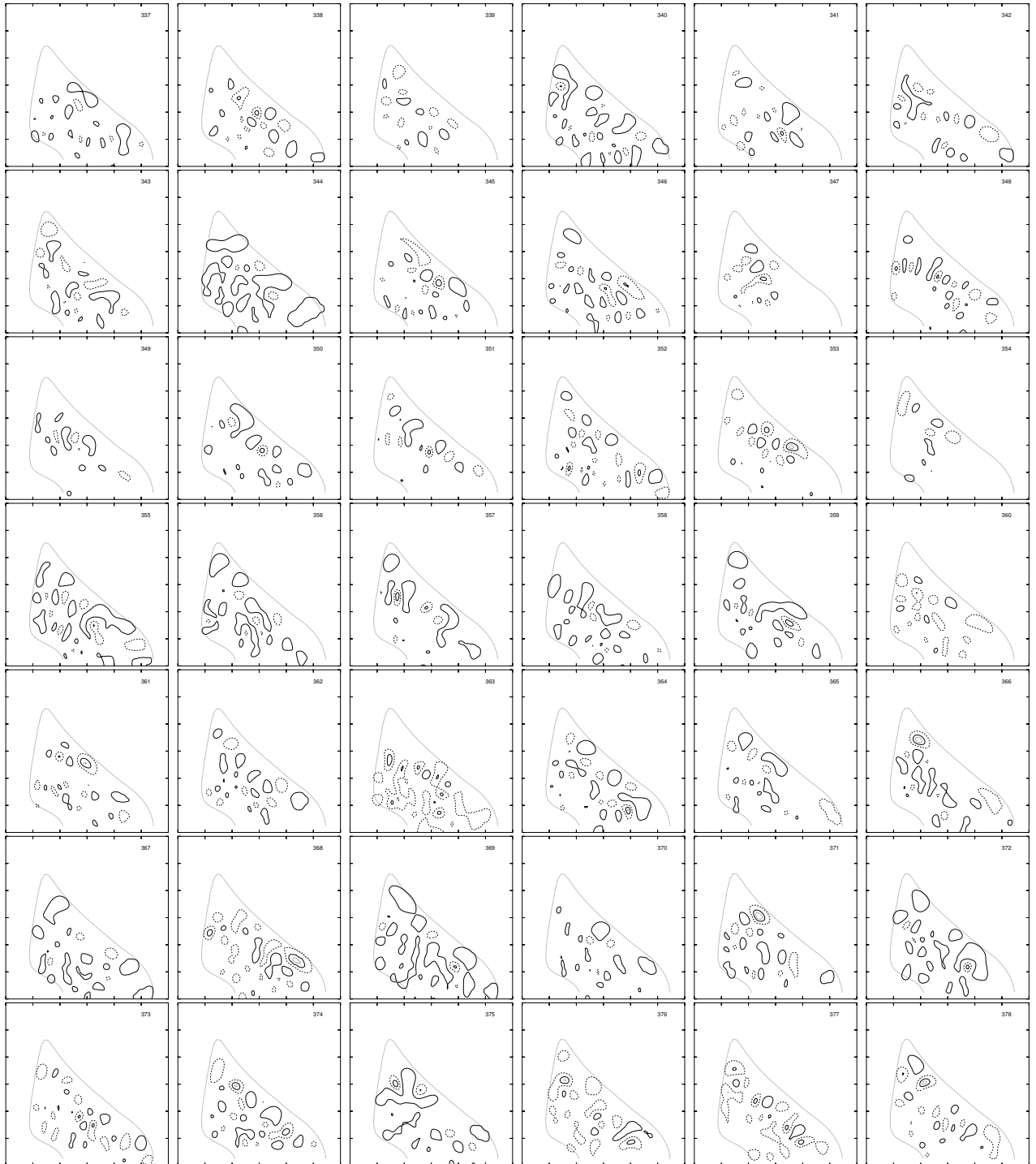
Figure 7.9: \text{H}_3^+ J = 0 even ( q = 0 ) wavefunctions in Jacobi (r_1, r_2, \theta) coordinates for states 337 to 378 with \theta taken to be 88.2^\circ . Contours are taken at 8%, 16%, 32% and 64% of the maximum amplitude. The dashed line enclosing each state indicates the classical turning point for that state. r_1 and r_2 are along the x and y axes respectively, with ranges from 0 to 6 a_0 .
