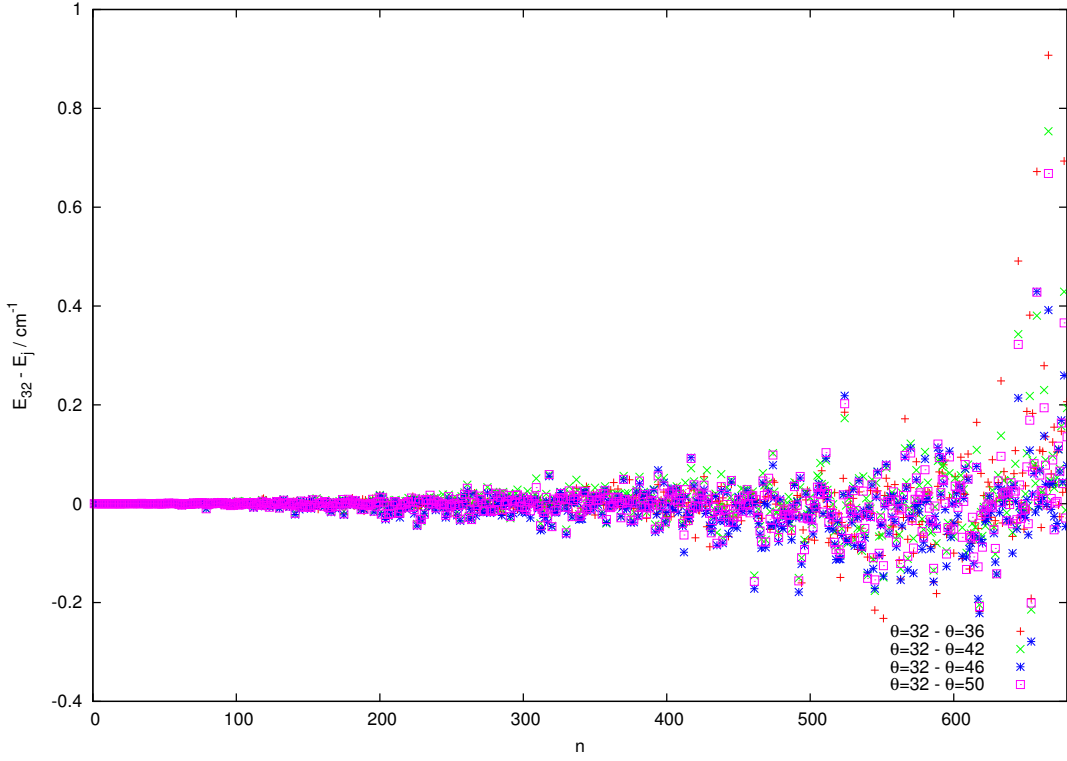
Figure 6.6: Convergence of J = 0 even band origins with respect to the value of n_\theta . The points indicate the difference of the n^{th} energy level calculated using a particular value of n_\theta relative to that calculated with n_\theta = 32
