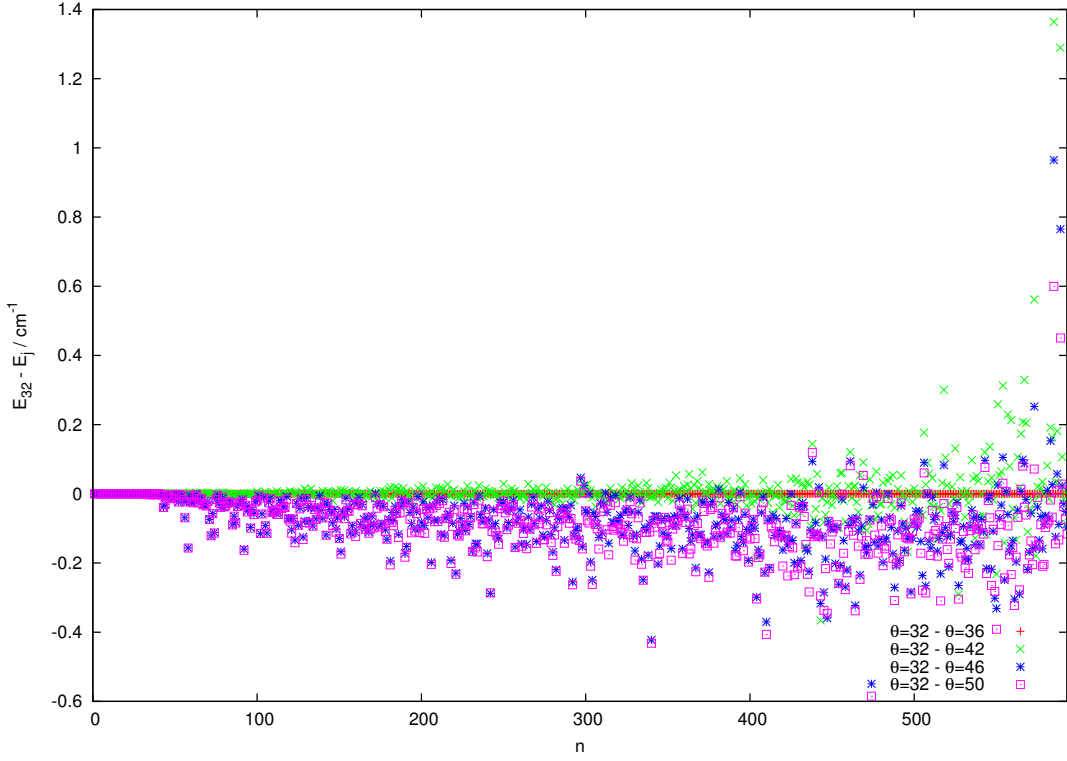
Figure 6.7: Convergence of J = 0 odd band origins with respect to the value of n_\theta . The points indicate the difference of the n^{th} energy level calculated using a particular value of n_\theta relative to that calculated with n_\theta = 32
