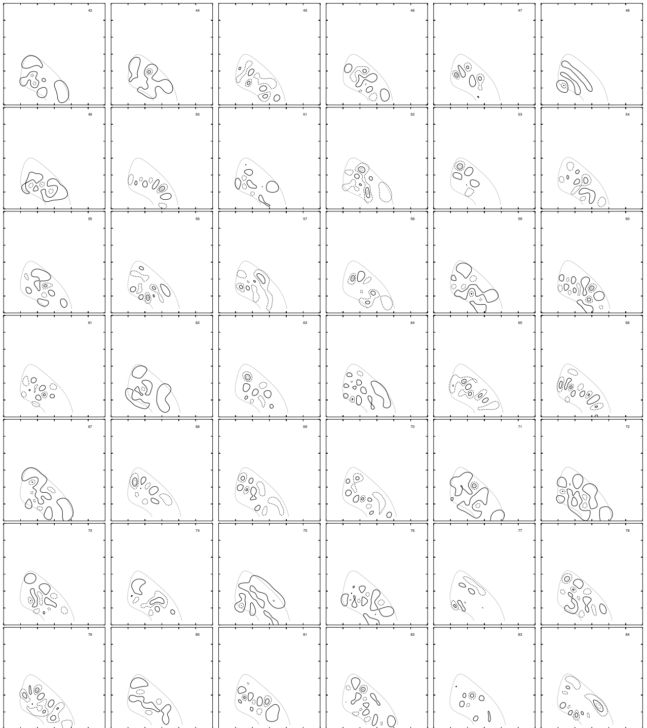
Figure 7.2: \text{H}_3^+ J = 0 even ( q = 0 ) wavefunctions in Jacobi (r_1, r_2, \theta) coordinates for states 43 to 84 with \theta taken to be 88.2^\circ . Contours are taken at 8%, 16%, 32% and 64% of the maximum amplitude. The dashed line enclosing each state indicates the classical turning point for that state. r_1 and r_2 are along the x and y axes respectively, with ranges from 0 to 6 a_0 .
