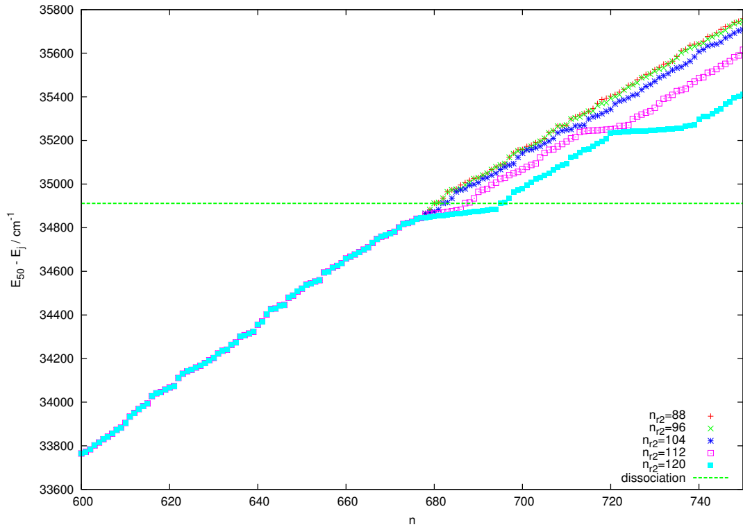
Figure 6.11: Convergence of J = 0 odd band origins with respect to the value of n_{r2} . The values of the other parameters are : N=29952 , n_{r1}=36 , n_{\theta} = 32 , \alpha = 0.0 , and \omega = 0.0075 .
